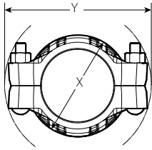
Style SC85 Joint Assembled 2 – 8"/DN50 – DN200
